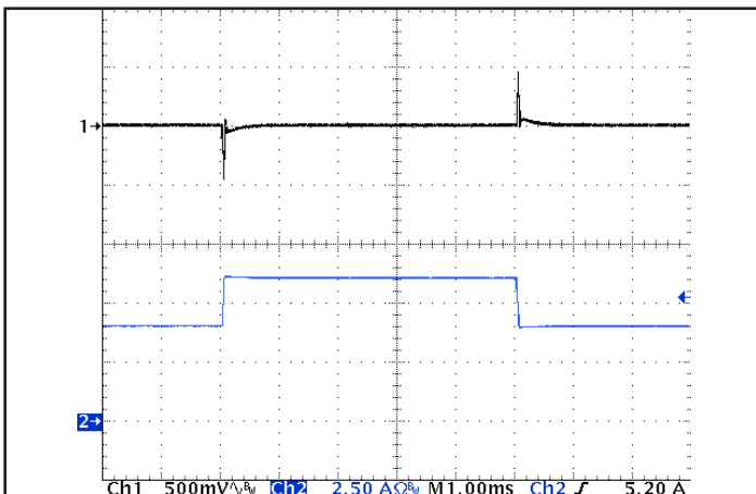
Figure 5: Output voltage response to step-change in load current (66% -100% -66% of I_{out(max)} ; dI/dt = 0.1 \text{ A}/\mu\text{s} ). Load cap: 1 \mu\text{F} ceramic and 15 \mu\text{F} tantalum capacitors. Ch 1: V_{out} (500 mV/div), Ch 2: I_{out} (2.5 A/div).
