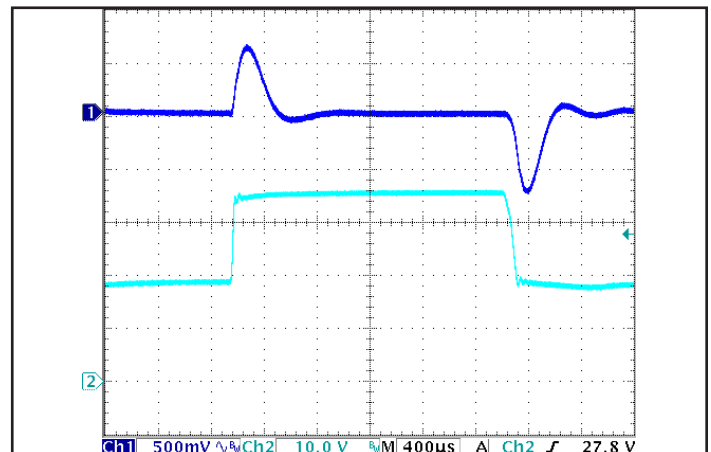
Figure 6: Output voltage response to step-change in input voltage (300 V/ms). Load cap: 100 \mu F , electrolytic output capacitance. Ch 1: V_{out} (500 mV/div), Ch 2: V_{in} (10 V/div).
