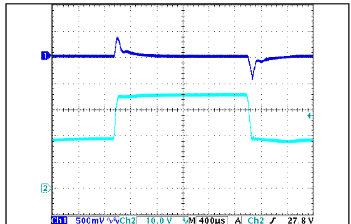
Figure 6: Output voltage response to step-change in input voltage (300 V/ms). Load cap: 100 \mu\text{F} , electrolytic output capacitance. Ch 1: V_{out} (500 mV/div), Ch 2: V_{in} (10 V/div).
