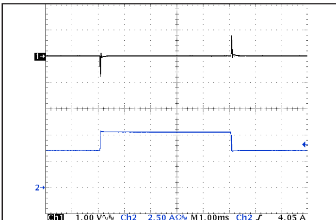
Figure 5: Output voltage response to step-change in load current (66% -100% -66% of Iout(max); dI/dt = 0.1 A/μs). Load cap: 1 μF ceramic and 15 μF tantalum capacitors. Ch 1: Vout (1 V/div), Ch 2: Iout (2.5 A/div).
